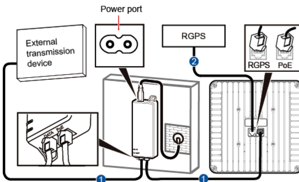
Figure 1-10 Cable connections
